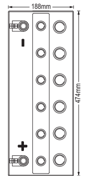
Battery Layout
